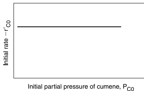
Figure 10-17 Desorption-limited reaction.
